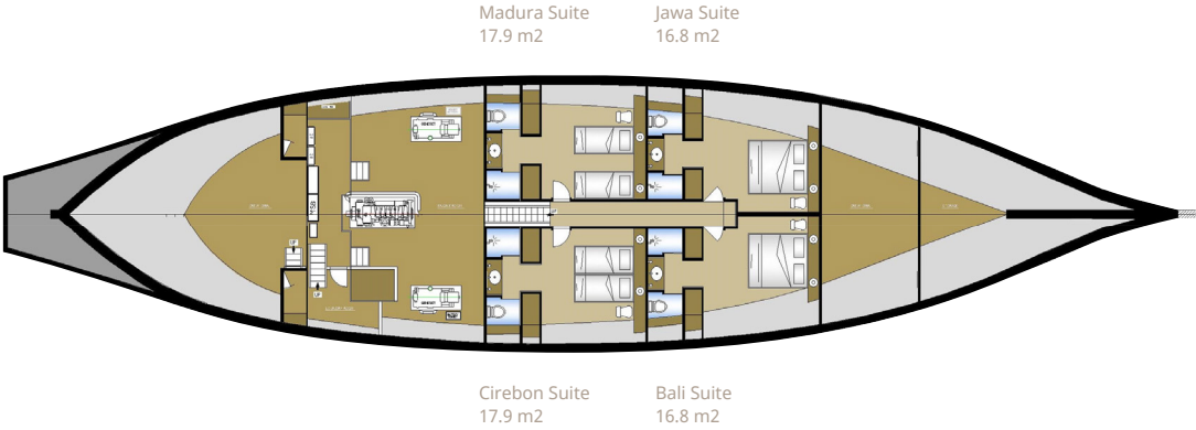
Lower Deck
